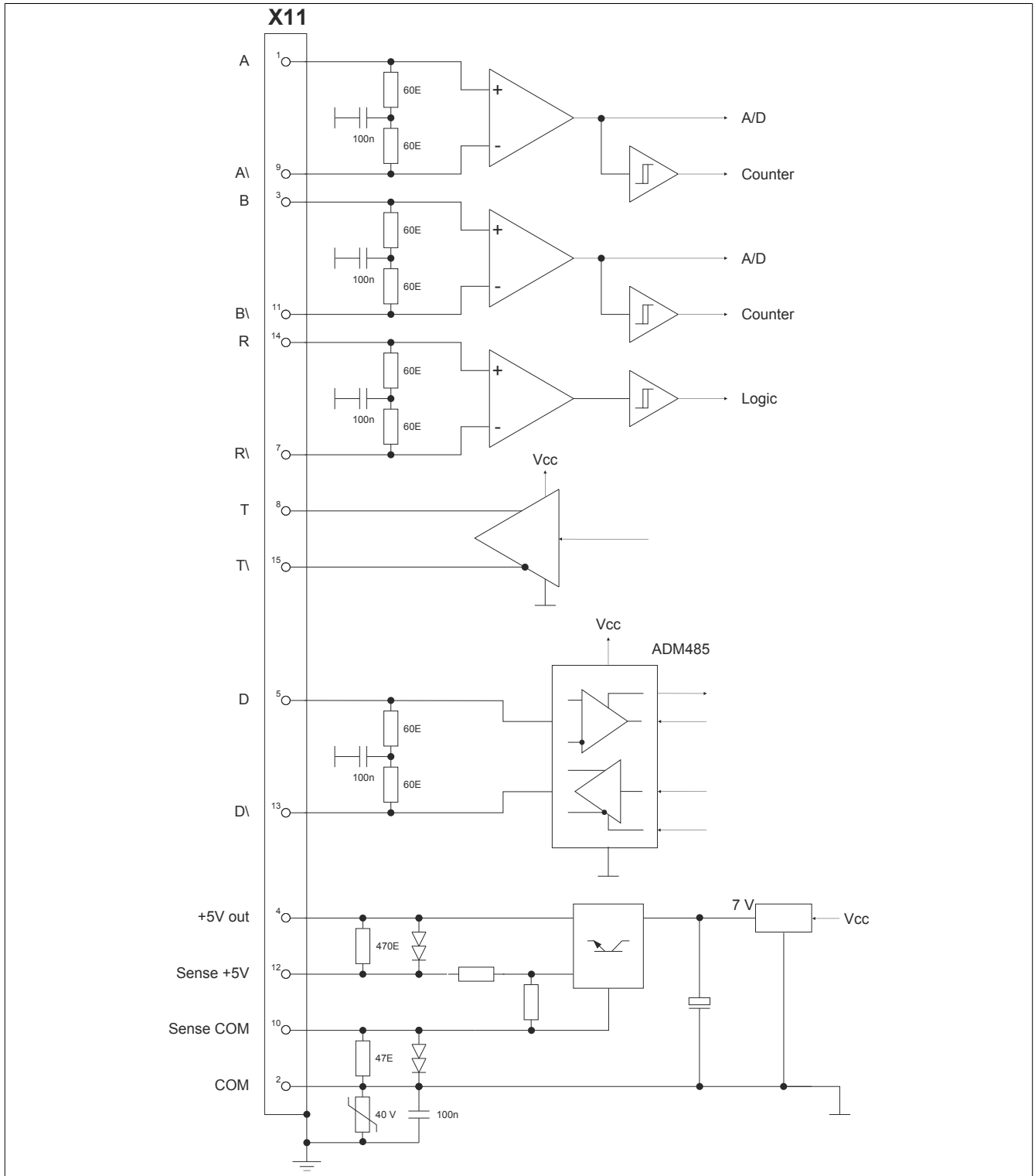
Figure 1: AC120 - Input/Output circuit diagram
